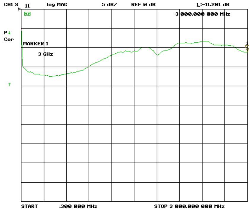
Picture 19 – TBWA2/40dB, input return loss, IS111, 300 kHz – 3 GHz, lin.
