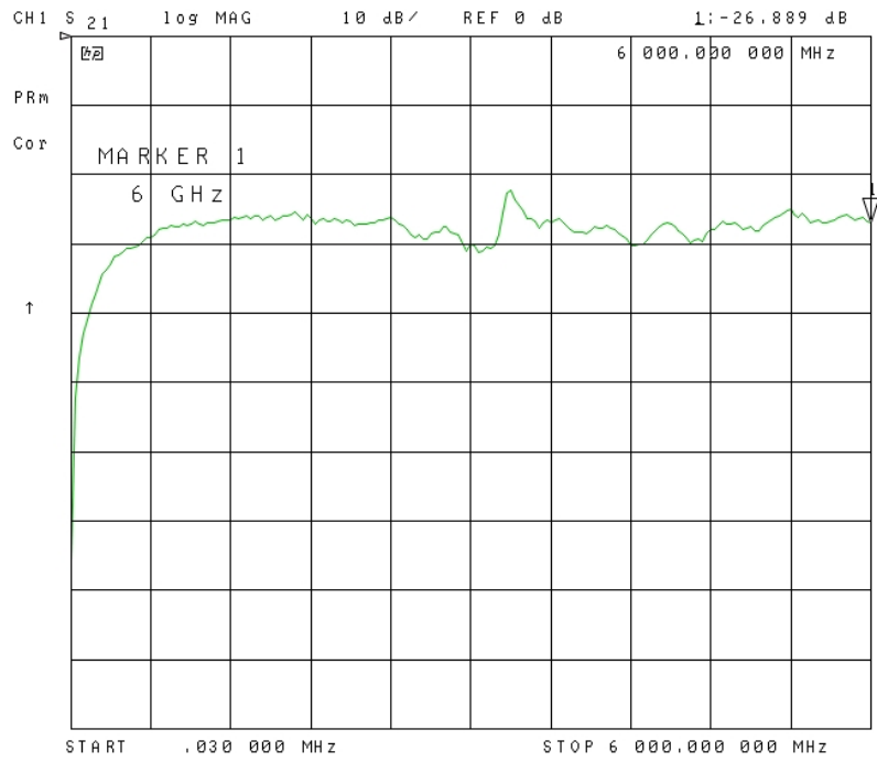
Picture 7 – H10, coupling loss, 30 kHz – 6 GHz, lin.
