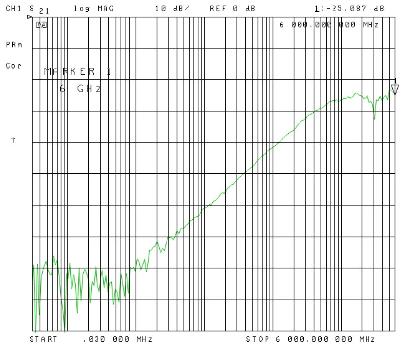
Picture 8 – H10, coupling loss, 30 kHz – 6 GHz, log.
