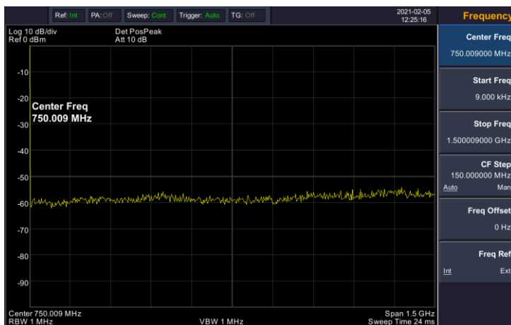
Figure 4-8 Full Span
