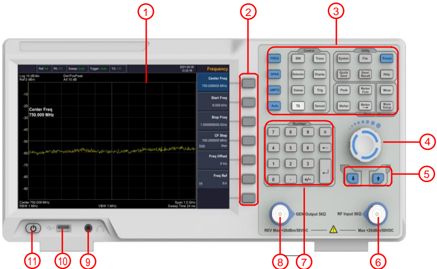
Figure 4-1 Front panel
