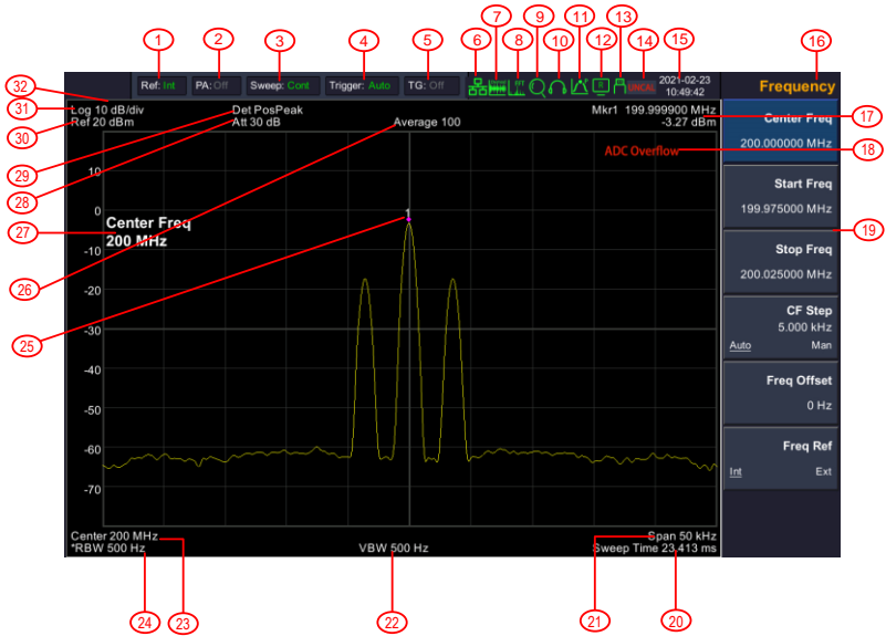
Figure 4-7 User interface
