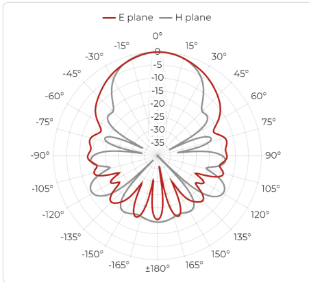
Port A, 8 GHz
