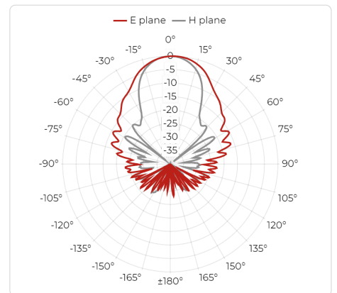
Port A, 18 GHz
