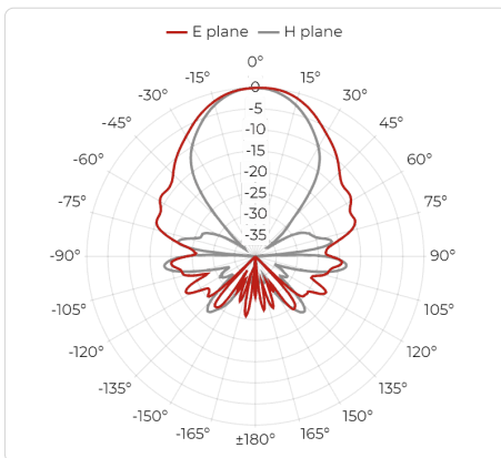
Port A, 14 GHz
