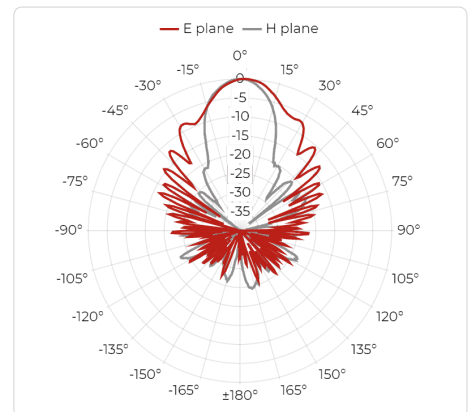
Port A, 18 GHz
