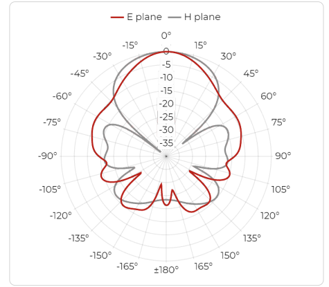
Port A, 6 GHz
