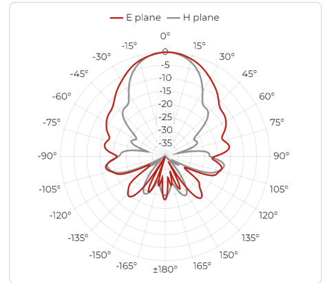
Port A, 12 GHz
