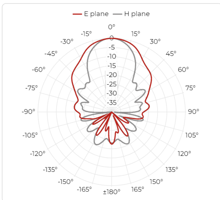
Port A, 4.8 GHz
