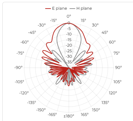
Port B, 5.4 GHz
