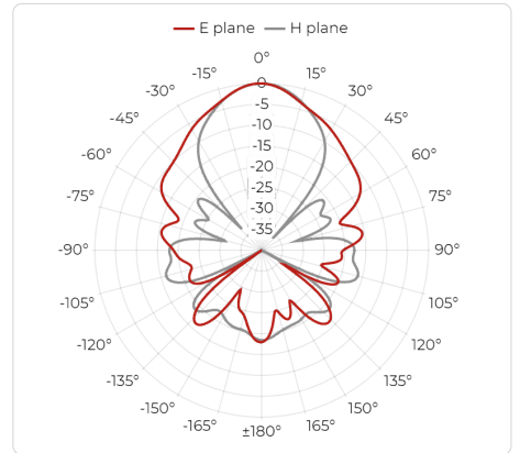
Port B, 4.2 GHz
