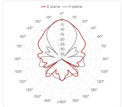
Port A, 4.2 GHz
