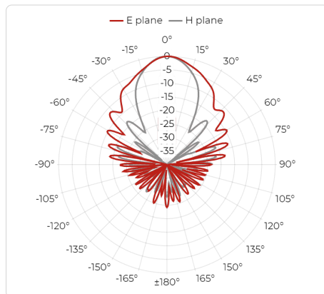
Port A, 5.4 GHz
