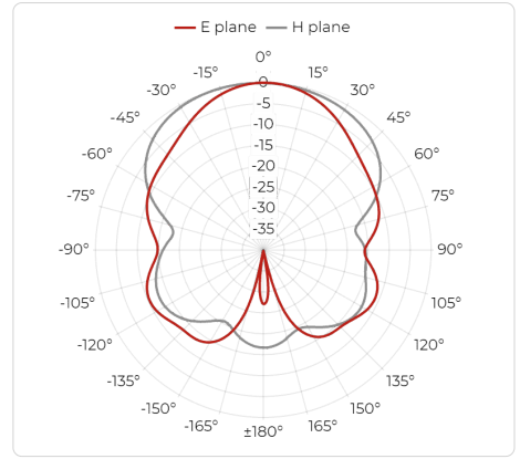
Port A, 2.4 GHz
