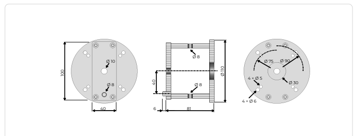
Mounting flange
