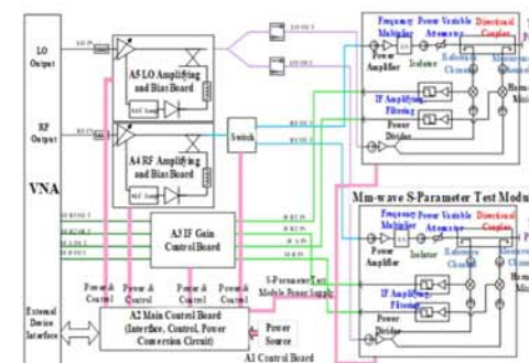
Fig. 1 Mm-wave and THz VNA System Schematic Diagram
