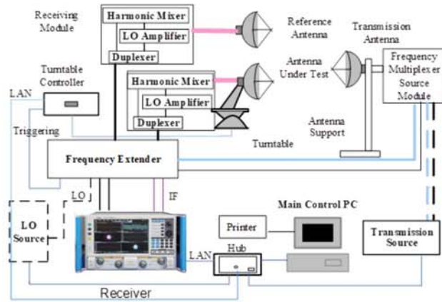
Fig. 11 Mm-wave and THz Antenna Test System Schematic Diagram
