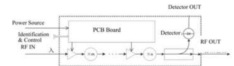
Fig. 4(b) Schematic Diagram – Source Extender Module with Amplitude Stabilization Option
