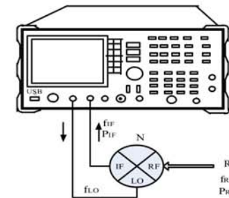
Fig. 6 Mm-wave and THz Spectrum Analysis System Schematic Diagram
