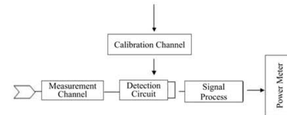
Fig. 8 Mm-wave and THz Power Sensor Schematic Diagram
