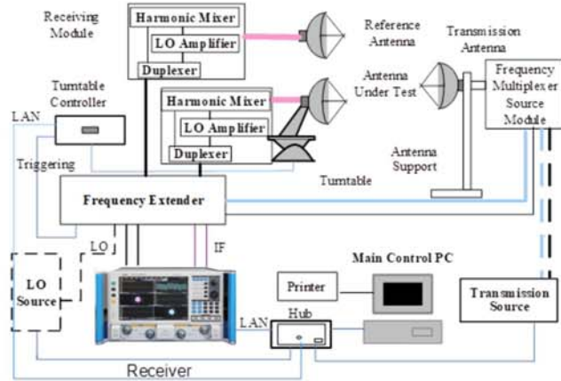
Fig. 12 Mm-wave and THz RCS Test System Schematic Diagram
