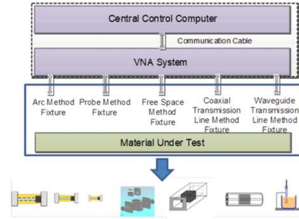
Fig. 13 Mm-wave and THz Material Test System Schematic Diagram
