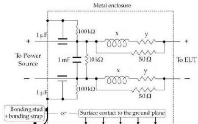
Figure 5.6.5-2: LISN schematic
