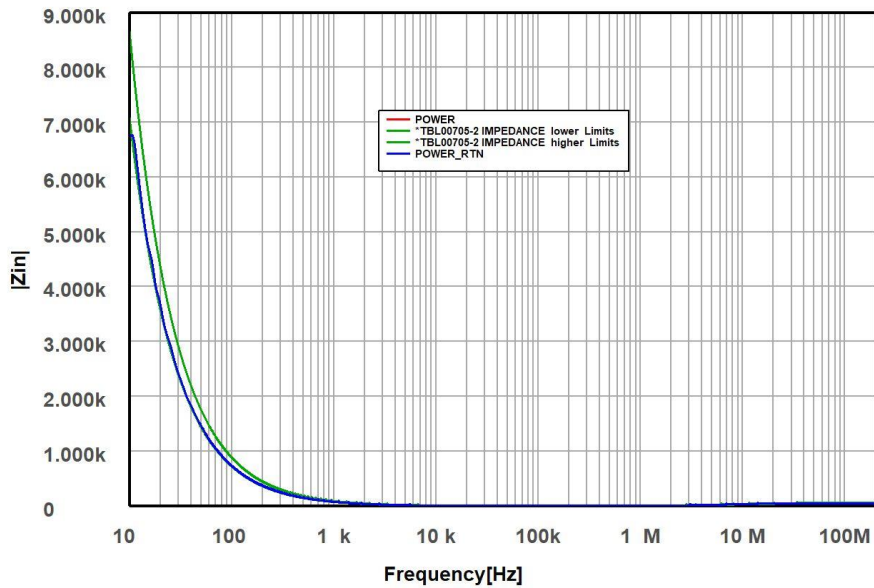
TBL00705-2 IMPEDANCE
