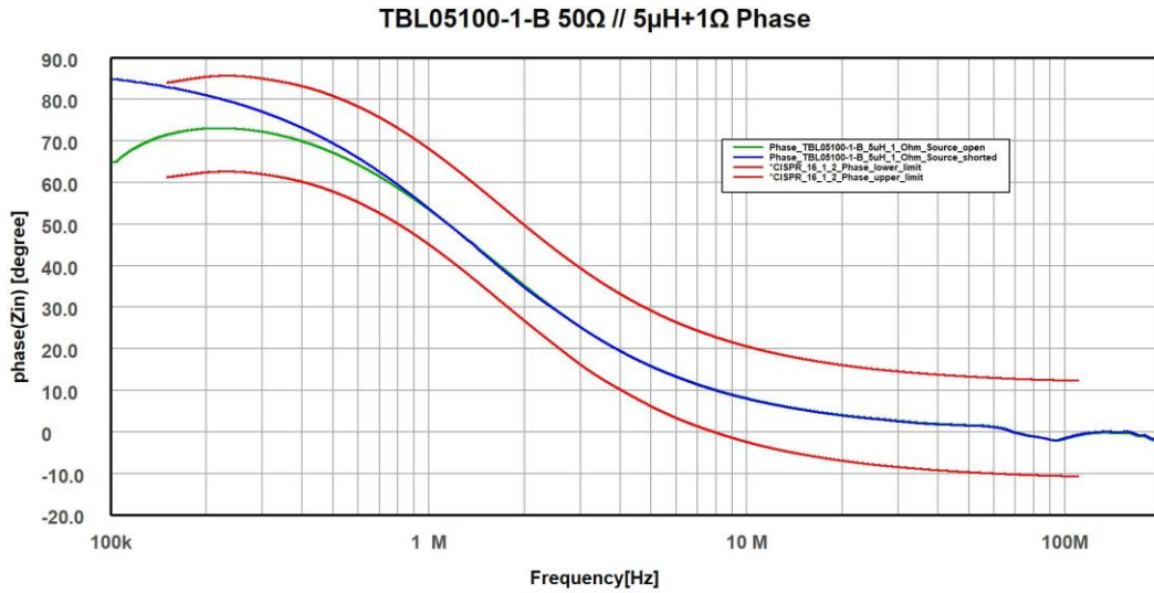
Picture 7: LISN phase, 100 kHz – 110MHz; 50Ω // 5μH+1Ω
