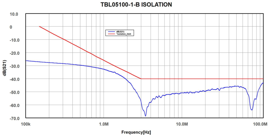
Picture 8: LISN Isolation, 100 kHz – 110MHz, 50Ω // 5μH+1Ω
