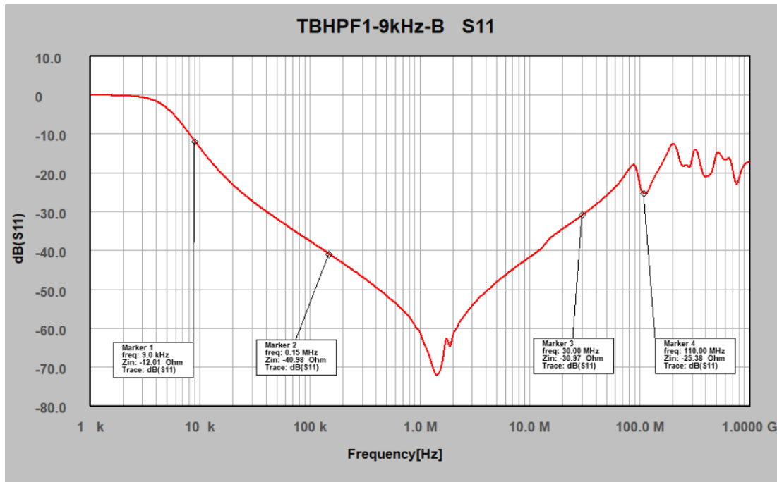
TBHPF1-9kHz-B: S11 (=S22), 1 kHz to 9 GHz, typical data
