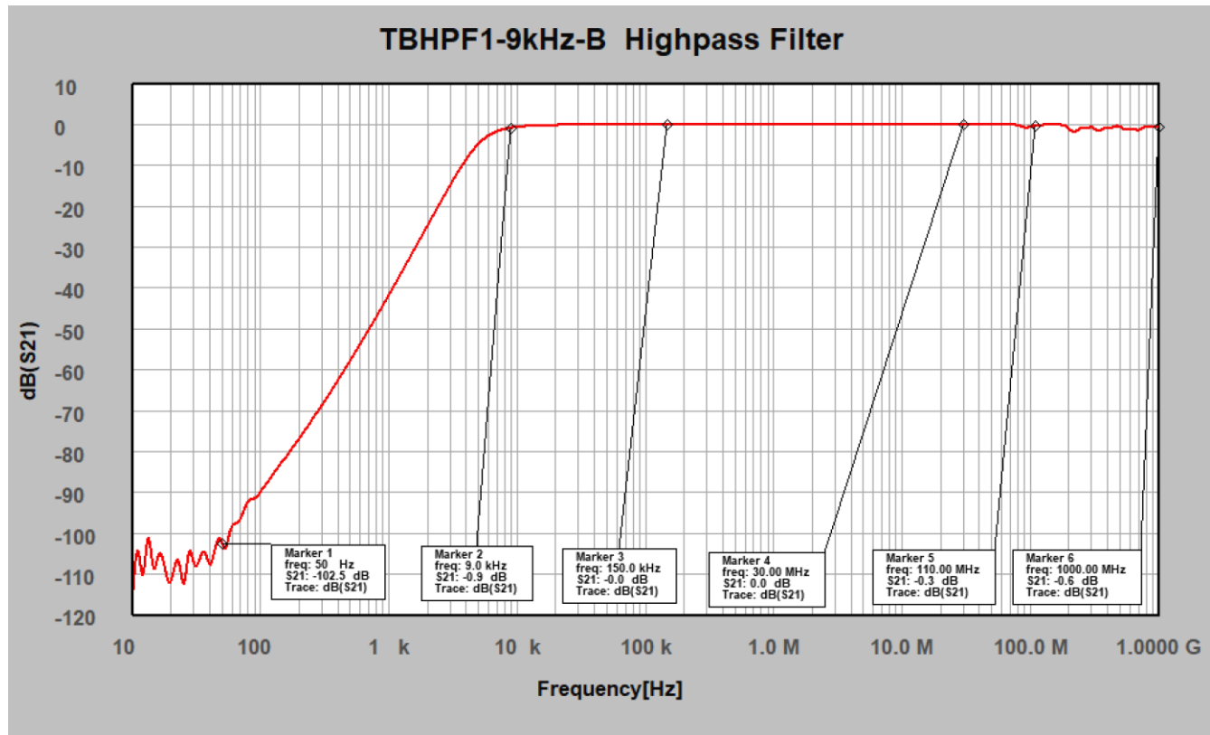
TBHPF1-9kHz-B: Insertion loss, 1 kHz to 1 GHz, typical data
