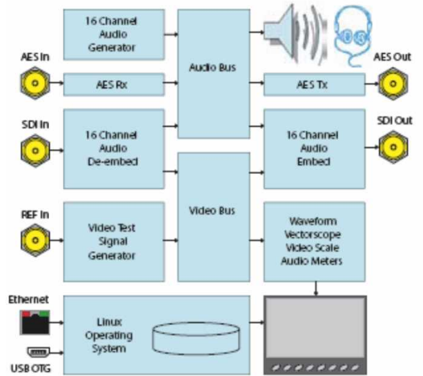
Schematic of the PHABRIX SxA (AES version)
