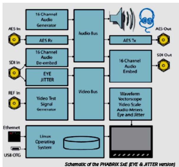
Schematic of the PHABRIX SxE (EYE & JITTER version)
