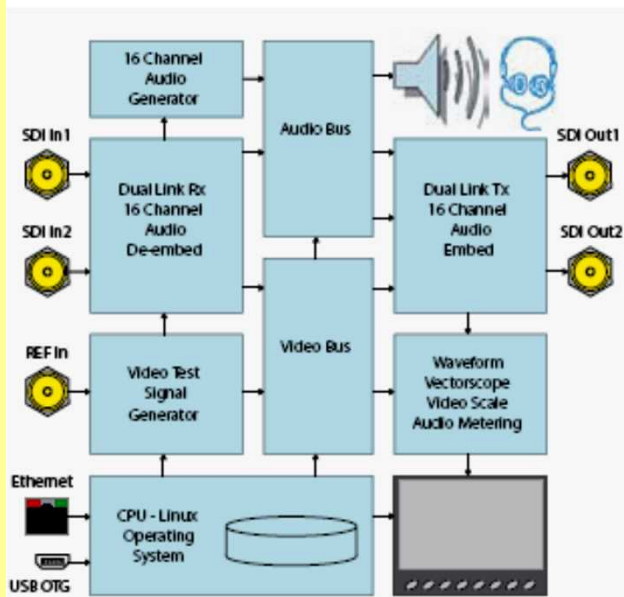
Schematic of the PHABRIX SxD (Dual Link version)
