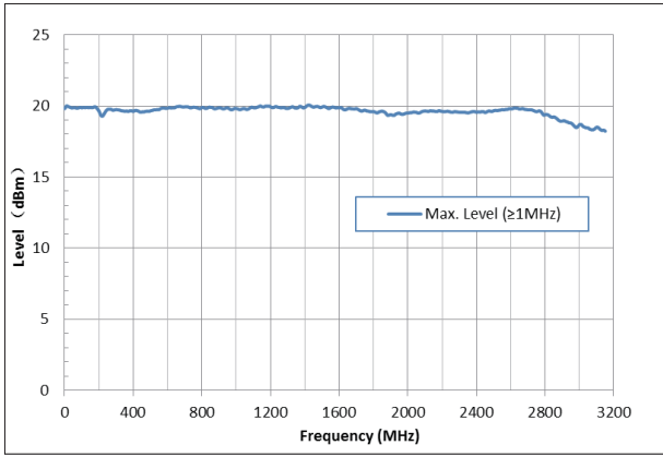
Maximum output power versus frequency, f \geq 1 MHz
